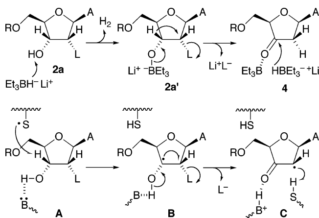
FIGURE 5. Comparison of [1,2]-hydride shift and [1,2]-electron shift (RNR) mechanisms.
