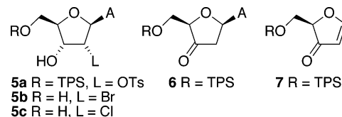
FIGURE 3. Precursor and possible product structures.
