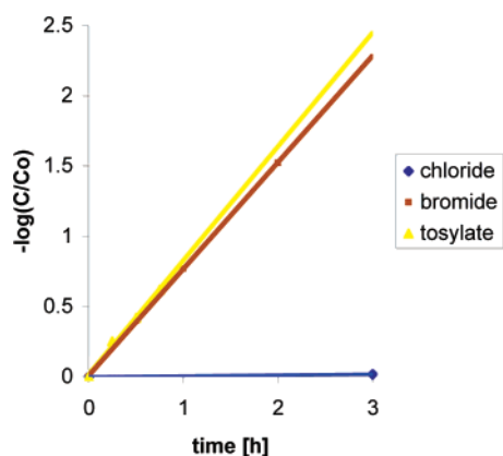
FIGURE 4. Pseudo-first-order plots for conversions of 2a , 5b , and 5c into 3a .
